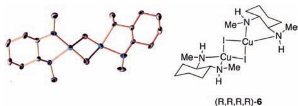
Figure 3. Crystal structure of the dimeric 1,2-diamine-ligated CuI complex.
