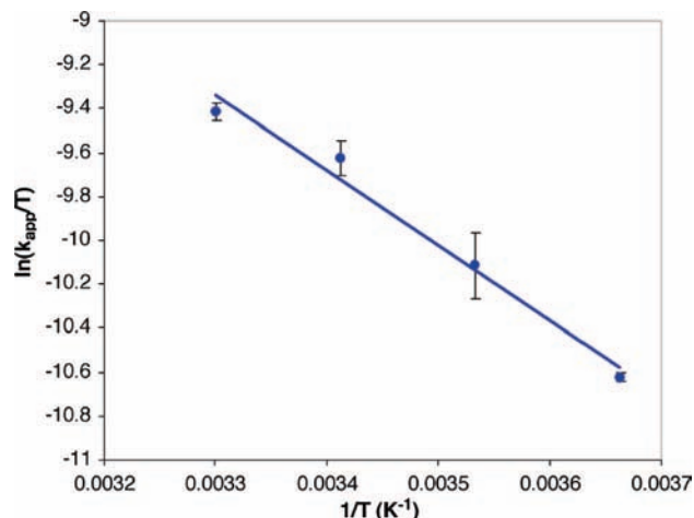
Figure 11. Eyring plot for the N -arylation of 8 (52 mM) with 1 (52 mM) in 1 mL of toluene from 0 to 30 °C. Each point is the average of three experiments.
