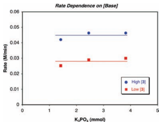
Figure 7. Dependence of the reaction rate on K₃PO₄ concentration at both (a) low [3] (Cu/3 = 1:2) and (b) high [3] (Cu/3 = 1:10). Conditions: (a) [3] = 0.04 M and (b) [3] = 0.2 M, [CuI] = 0.02 M, [I]₀ = 0.4 M, [2]₀ = 0.83 M, [K₃PO₄]₀ = 1.4–3.8 mmol, 2 mL of toluene, 90 °C.
