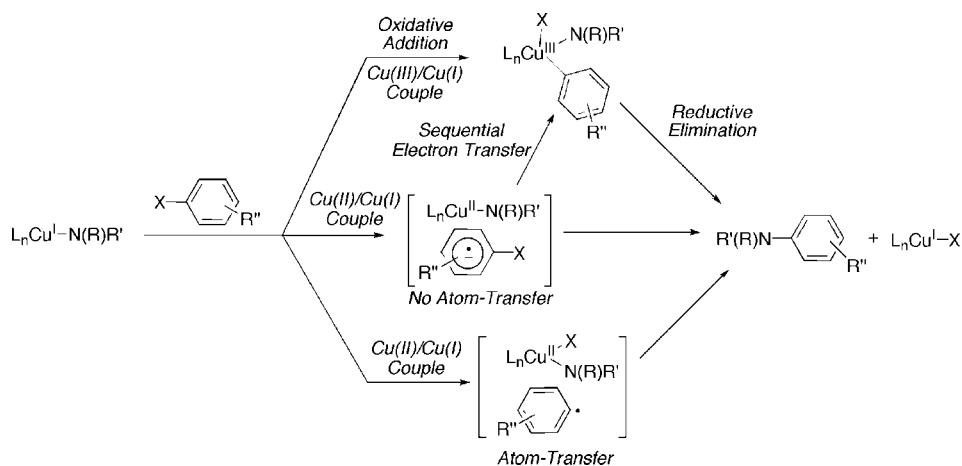
Scheme 3. Possible Mechanisms for the Cu(I) Amidate Promoted Aryl Iodide Activation
