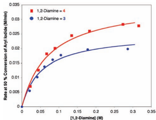
Figure 2. Reaction rate at 50% conversion of 1 vs [1,2-diamine] in the N -arylation of 2 (0.8 M) with 1 (0.4 M) using [CuI] (0.02 M) at 90 °C. The curve fit reflects a nonlinear least-squares fit to a function: rate = C 1 [1,2-diamine]/(C 2 + [1,2-diamine]).
