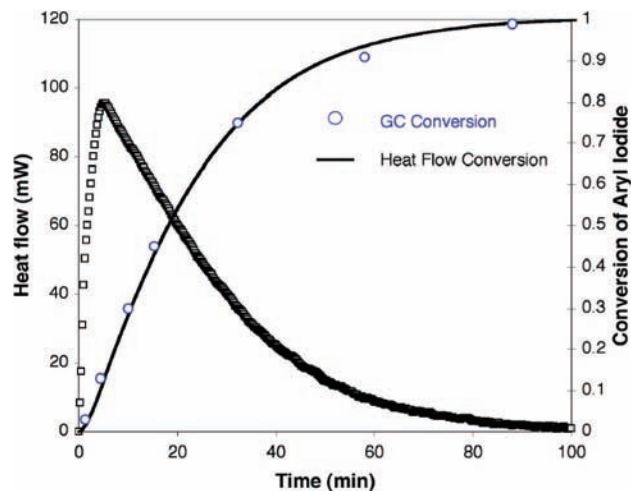
Figure 1. Representative heat flow versus time profile for the CuI/3 catalyzed N -arylation of 2-pyrrolidinone with 3,5-dimethyliodobenzene and comparison of conversion data obtained from heat flow to that obtained by GC measurements. Data sampling occurred at a rate of 4 min -1 . Conditions: [1] 0 = 0.4 M, [2] 0 = 0.8 M, [K 3 PO 4 ] 0 = 2.4 mmol, 25 [CuI] = 0.02 M, [3] = 0.04 M in 2.0 mL of toluene at 90 °C.
