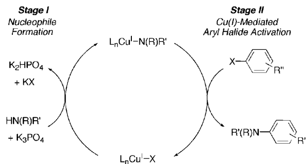
Scheme 1. Simplified Catalytic Cycle Displaying the Two-Stage Cu(I)-Catalyzed N -Arylation Process
