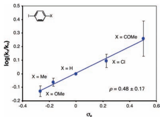
Figure 8. Hammett plot derived from the observed rate constants of the N -arylation of 2-pyrrolidinone (2) with a series of para -substituted aryl iodides. Conditions: [CuI] = 0.02, [3] = 0.04 and 0.2 M, [aryl iodide]₀ = 0.4 M, [2]₀ = 0.83 M, [K₃PO₄]₀ = 2.4 mmol, 2 mL of toluene, 90 °C. Each point is the average of six experiments: three experiments at each high and low [3].
