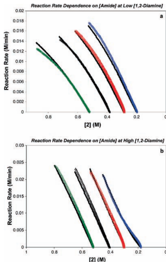
Figure 5. Dependence of the reaction rate on amide concentration ([ 2 ]) at both (a) low [ 3 ] (Cu/ 3 = 1:2) and (b) high [ 3 ] (Cu/ 3 = 1:10). Conditions: (a) [ 3 ] = 0.04 M and (b) [ 3 ] = 0.2 M, [CuI] = 0.02, [ 1 ] 0 = 0.4 M, [ 2 ] 0 = 0.93 M (green times signs), 0.8 M (black times signs), 0.7 M (red squares), 0.6 M (blue times signs), [K 3 PO 4 ] 0 = 2.4 mmol, 2 mL of toluene, 90 °C. The black curves represent the nonlinear least-squares fit to eq 9. The kinetic parameters are as follows: K_1 = 0.85 \pm 0.05 , K_2 = 2.0 \pm 0.2 , k_{\text{act}} = 12 \pm 3 \text{ M}^{-1} \cdot \text{min}^{-1} .
