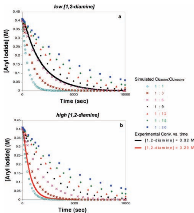
Figure 15. Comparison between experimental conversion vs time data and results obtained by numerically integrating eq 14 with k_{app} = 0.20 \text{ M}^{-1} \cdot \text{s}^{-1} for different ratios of k_f/k_r ( = \text{Cu}_{active}/\text{Cu}_{inactive} ). Conditions: [\text{ArI}]_0 = 0.4 \text{ M} , [\text{Cu}_{inactive}]_0 = 0.02 \text{ M} , (a) experimental [\text{3}] = 0.02 \text{ M} , (b) experimental [\text{3}] = 0.29 \text{ M} .
