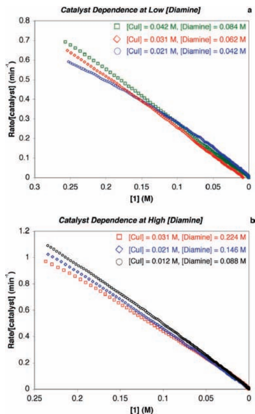
Figure 4. Dependence of the reaction rate on catalyst concentration at both (a) low [ 3 ] (Cu/ 3 = 1:2) and (b) high [ 3 ] (Cu/ 3 = 1:7). In both cases the reaction rate displays a first-order dependence on catalyst concentration, i.e., \text{rate} \propto [\text{catalyst}] or \text{rate}/[\text{catalyst}] = \text{constant} . Conditions: [CuI] = 0.01–0.04 M, [ 3 ] = 0.04–0.22 M, [ 1 ] 0 = 0.4 M, [ 2 ] 0 = 0.8 M, [K 3 PO 4 ] 0 = 2.4 mmol, 2 mL of toluene, 90 °C.
