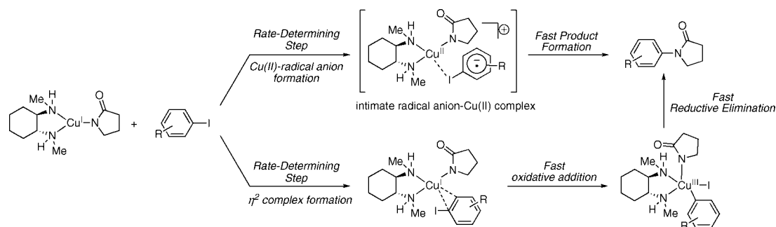
Scheme 3. Possible Mechanisms for the Cu(I) Amidate Promoted Aryl Iodide Activation
