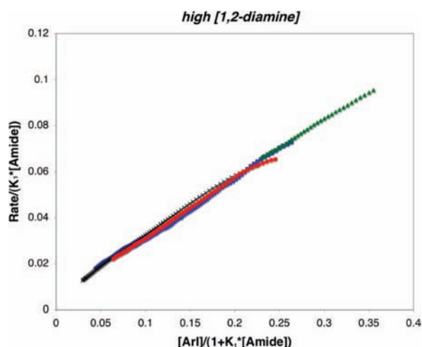
Figure 14. The quasilinear relationship between rate/ K_1[\text{amide}] and [\text{ArI}]/(1 + K_1[\text{amide}]) , where K_1 is 0.85 \pm 0.05 , is shown based on eq 13. The slope, which is equal to k_{\text{act}}[\text{Cu}]_t , is 0.25 \pm 0.02 \text{ min}^{-1} . Conditions: high [3] (70 mol % 3 , 5 mol % CuI), (green triangles) [\text{2}]_0 = 0.8 \text{ M} , [\text{1}]_0 = 0.8 \text{ M} , (red circles) [\text{2}]_0 = 0.9 \text{ M} , [\text{1}]_0 = 0.6 \text{ M} , (blue squares) [\text{2}]_0 = 1.0 \text{ M} , [\text{1}]_0 = 0.6 \text{ M} .
