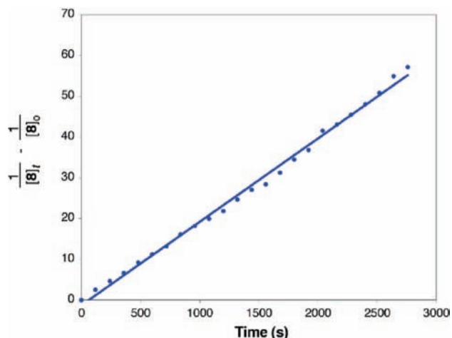
Figure 10. Linear relationship between 1/[8]_t - 1/[8]_0 and time (s) for the N -arylation of 8 (52 mM) with 1 (52 mM) in 1 mL of d_8 -toluene at 20 °C; k_{app} = 2.04 \times 10^{-2} \text{ M}^{-1} \cdot \text{s}^{-1} .
